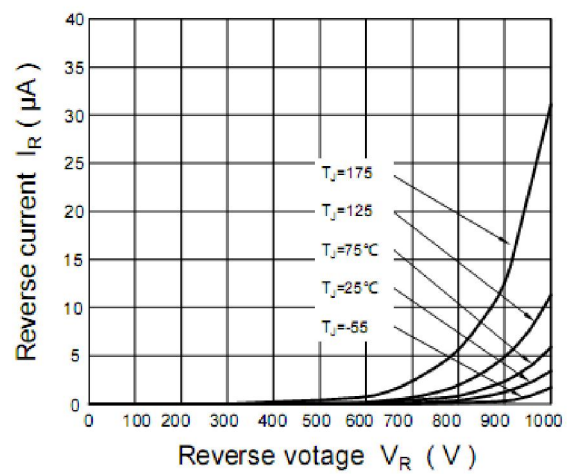
Figure 2. Reverse Characteristics
