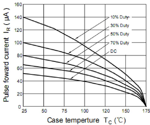
Figure 3. Current Derating
