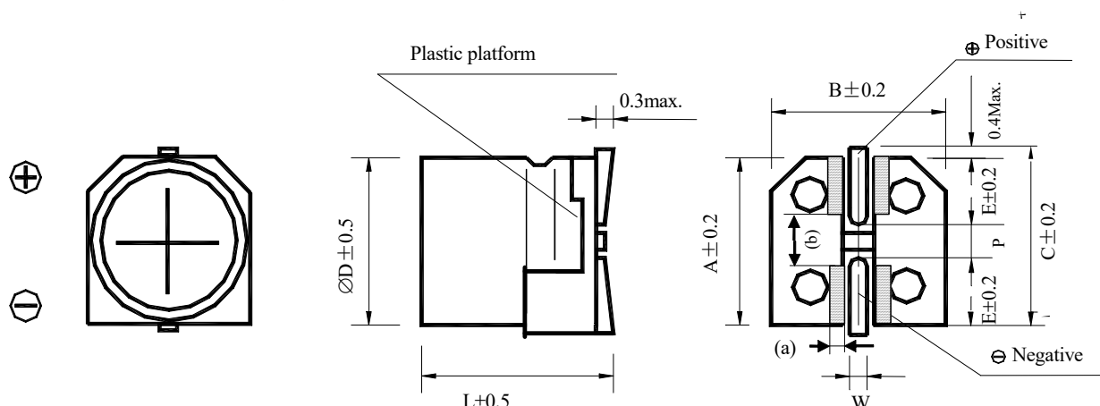
16. 尺寸: Dimensions (Unit: mm)
