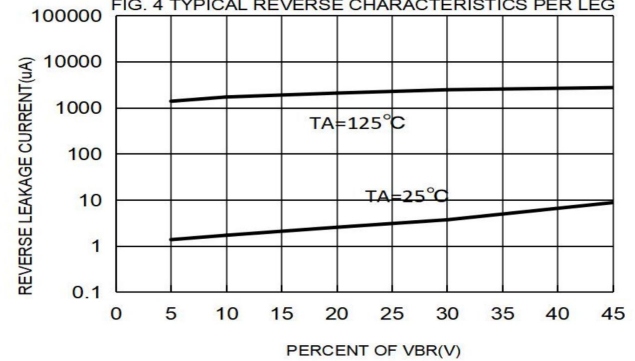
FIG. 4 TYPICAL REVERSE CHARACTERISTICS PER LEG
