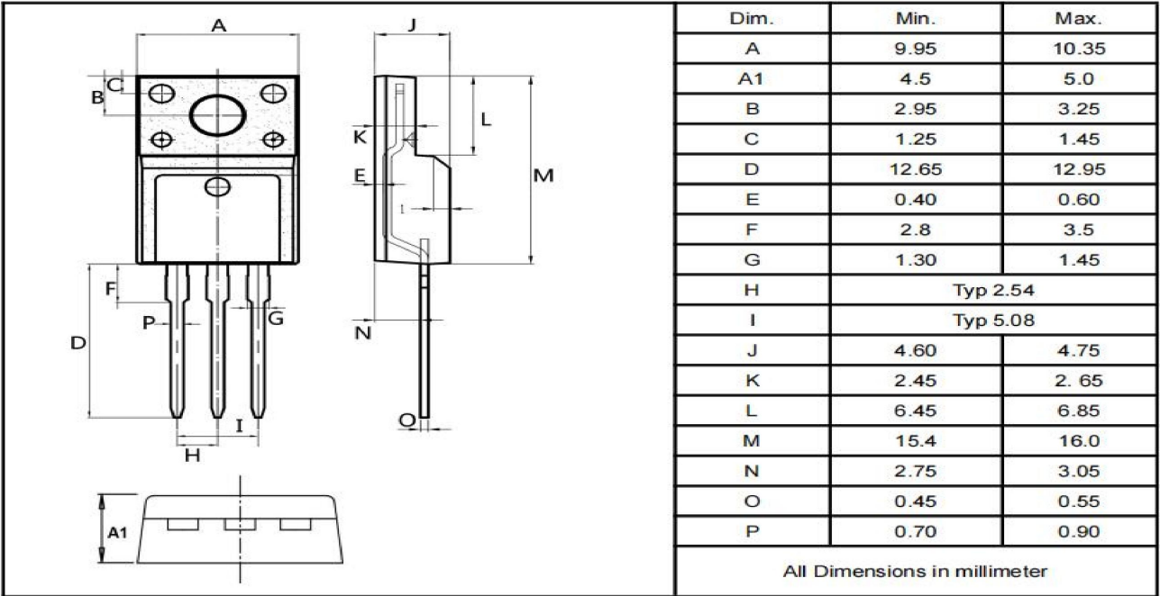
TO-220F
