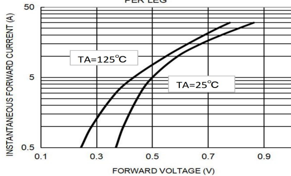
FIG. 3 TYPICAL FORWARD CHARACTERISTICS PER LEG
