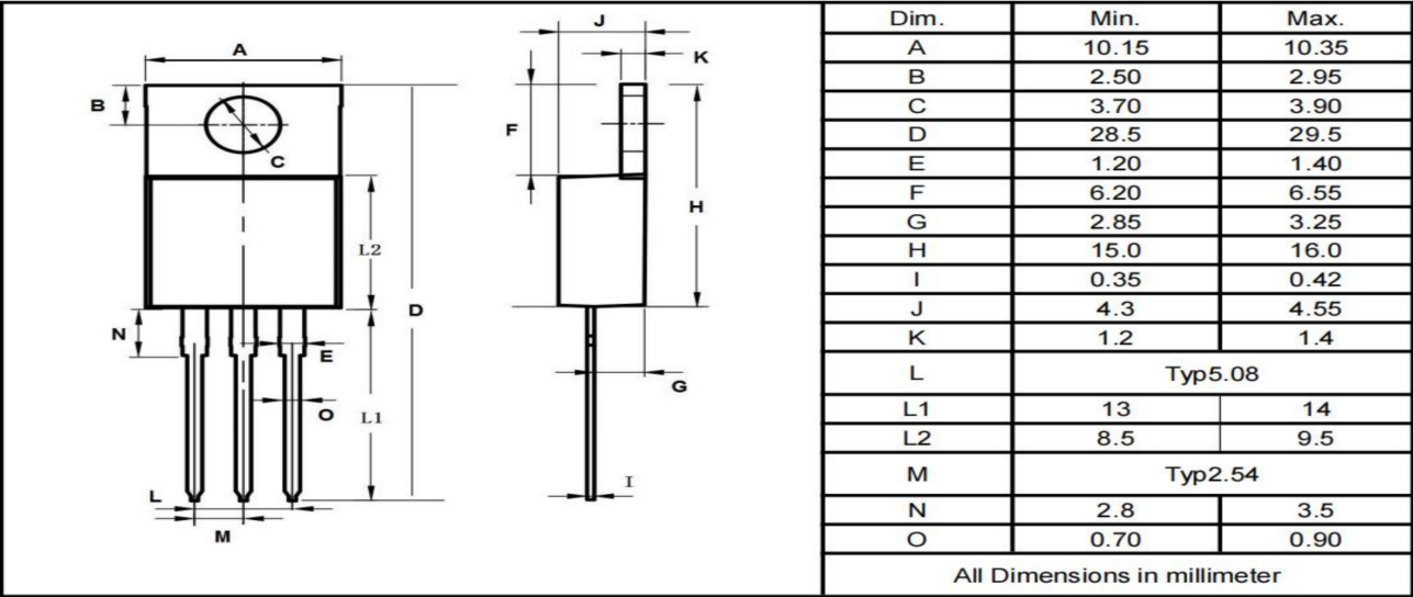
TO-220F
