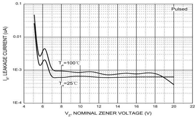
Fig.3 Typical Leakage Current
