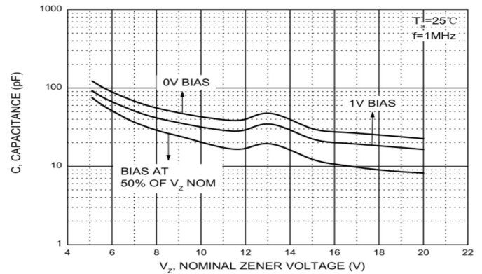
Fig.4 Typical Capacitance
