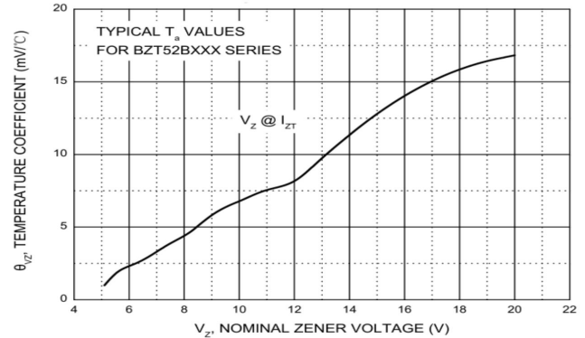
Fig.2 Temperature Coefficients
