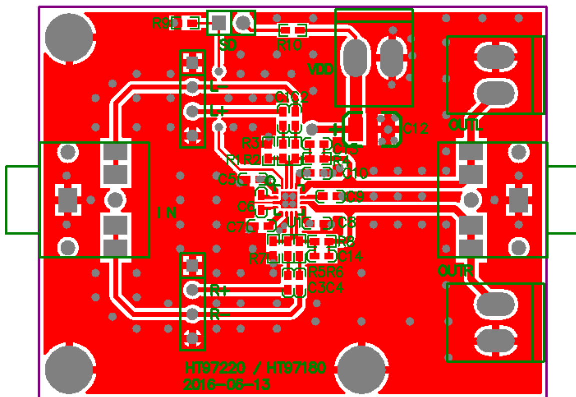
Fig.6 Top View of HT97220(L) Demo Board PCB Layout
