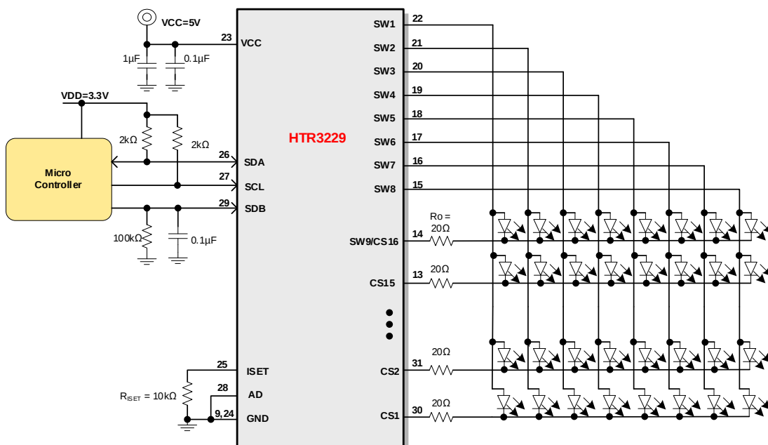
Driving 16×8 LEDs
