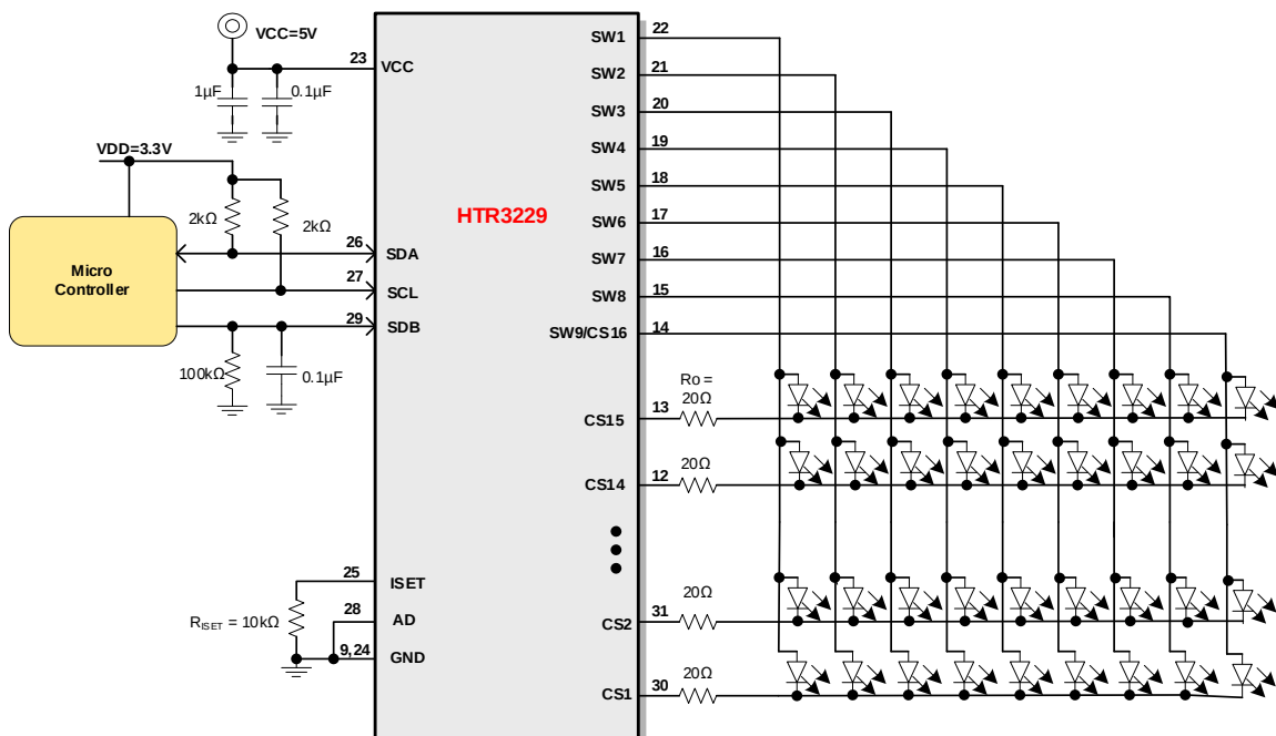
Driving 15×9 LEDs
