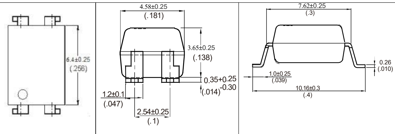
4-pin SMD
