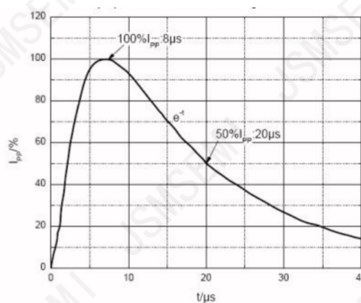
8/20µs pulse waveform according to IEC 61000-4-5
