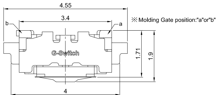
Actuator cross section(Section C-C)
