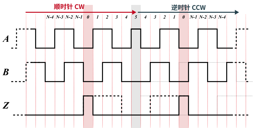
Figure 11: ABZ 输出时序
