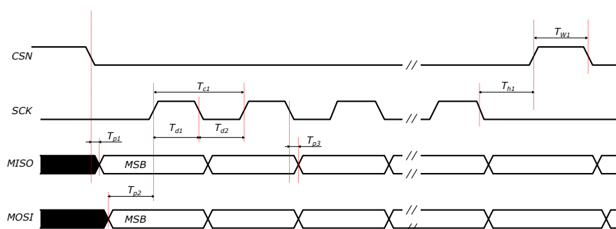
Figure 7: SPI 时序图
