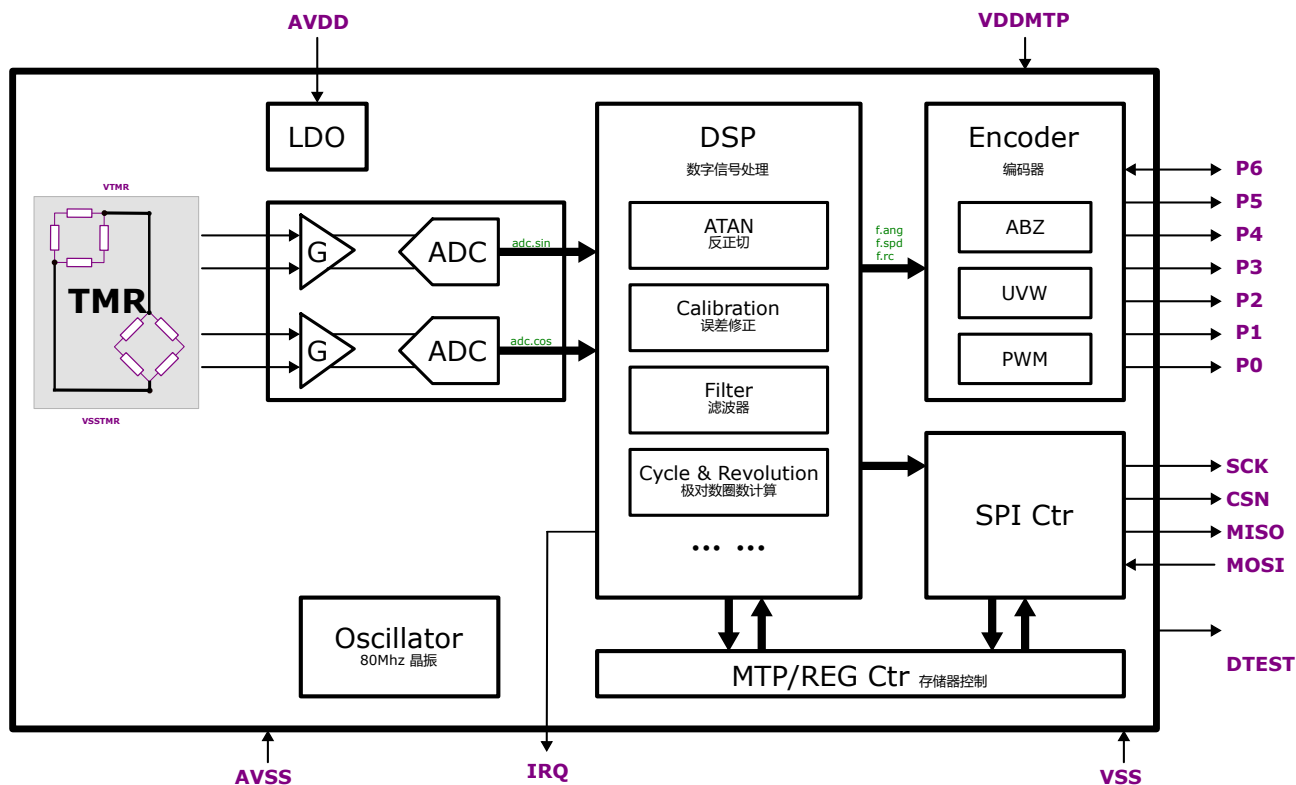
Figure 1: KTM5900 芯片功能框图
