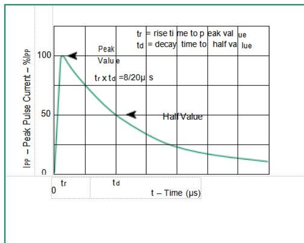
Figure 8 - Pulse Waveform
