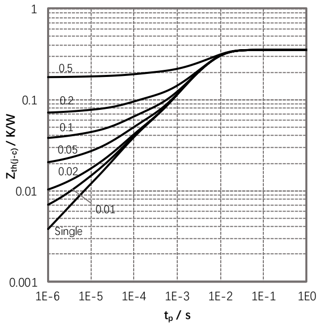
Fig 25. Transient Thermal Impedance
