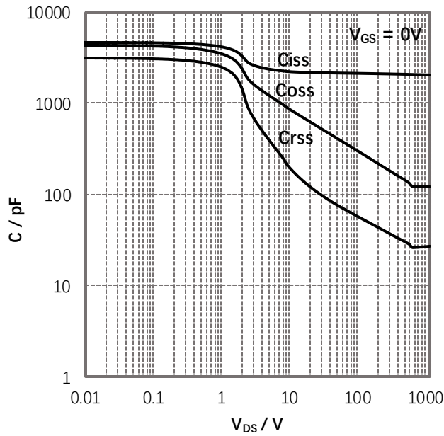
Fig 15. Capacitance Characteristics
