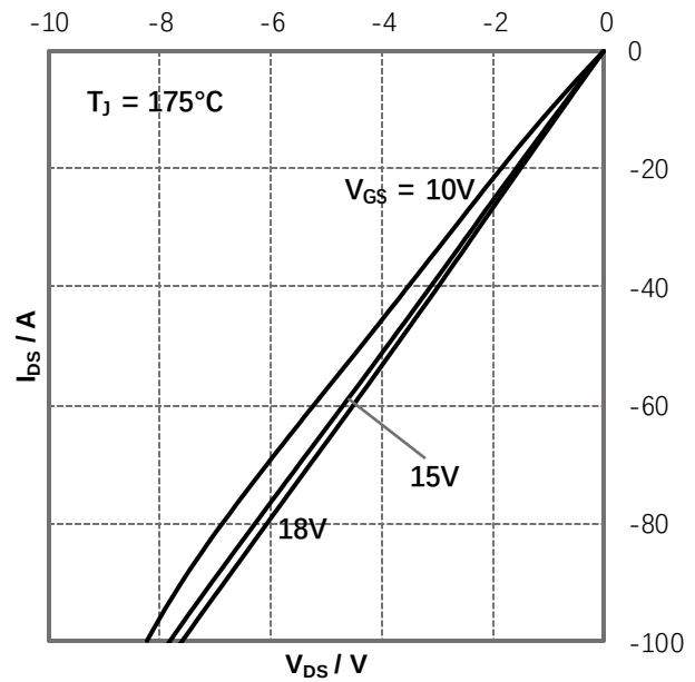
Fig 14. 3rd Quadrant Characteristics ( T_j = -175^\circ\text{C} )
