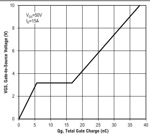
Figure 12. Gate-Charge Characteristics
