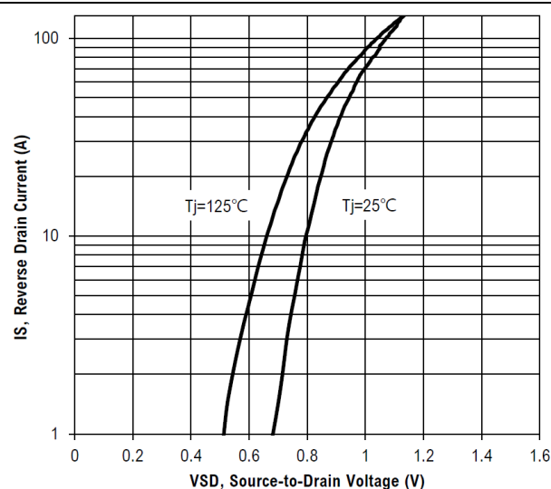
Figure 8. Body-Diode Characteristics
