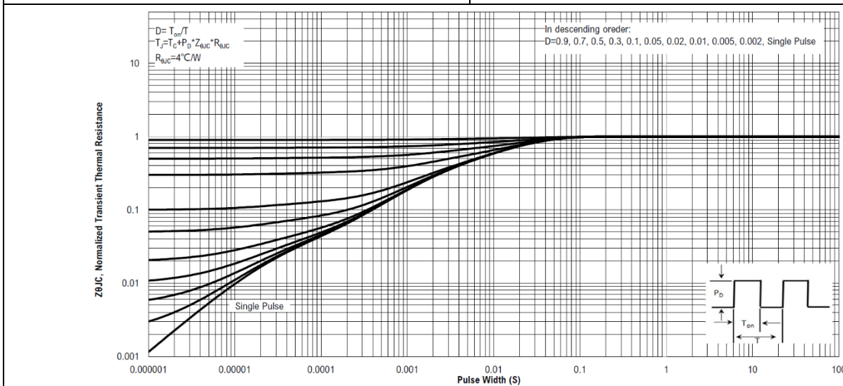
Figure 13. Transient Thermal Resistance
