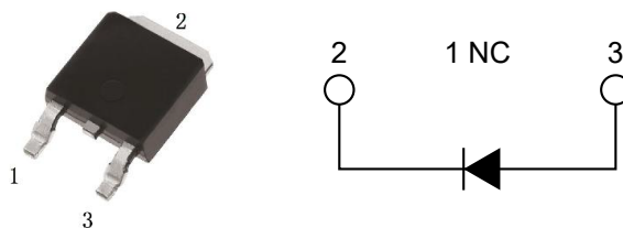
TO-252
