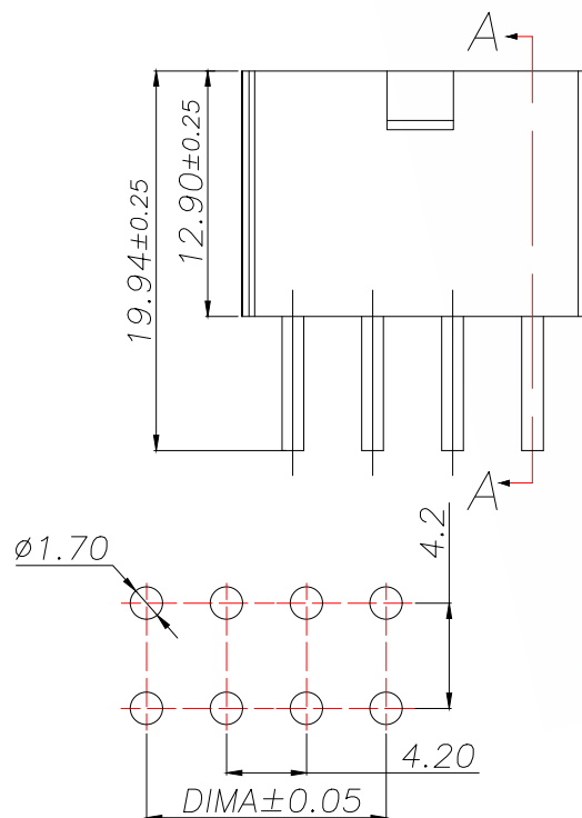
PCB.WELDING DRAWING (TOLERANCE:±0.05)
