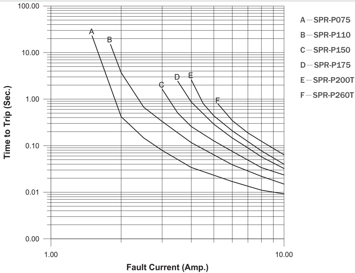
Average Time-Current Curve
