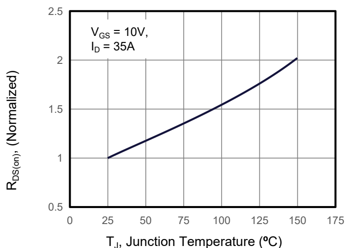
Figure 7. Drain-Source On-Resistance
