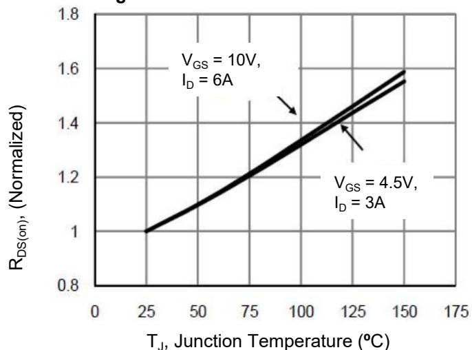
Figure 7. Drain-Source On-Resistance
