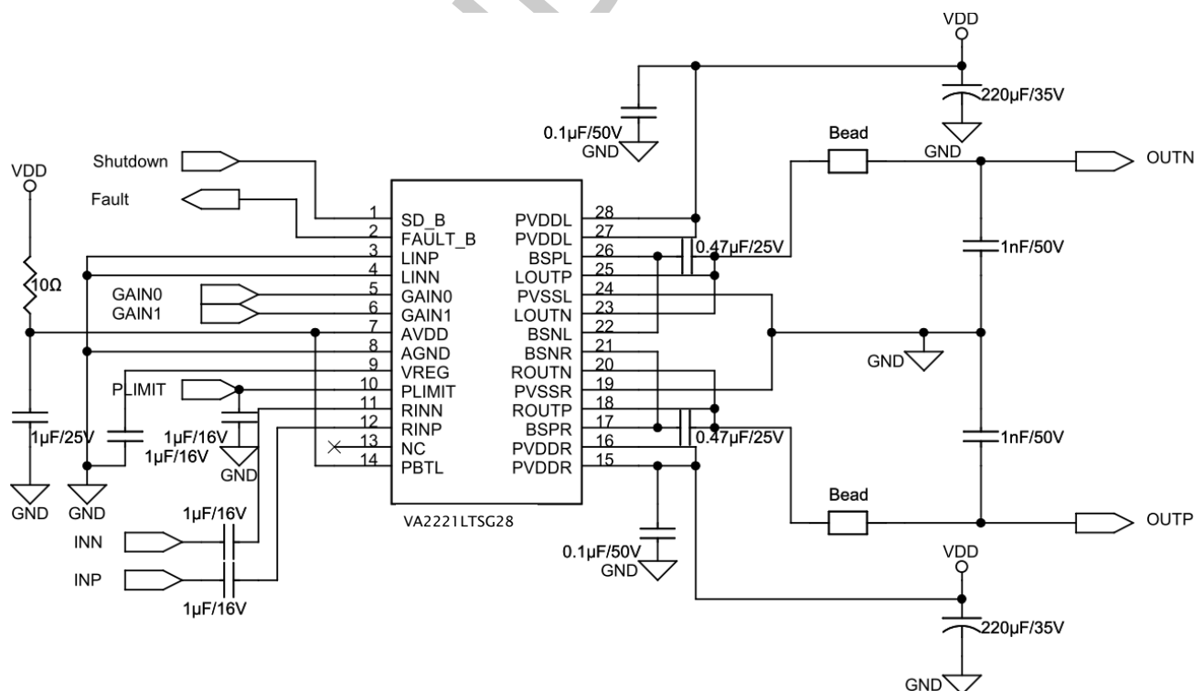
Figure 6. VA2221L Mono Reference Application with Ferrite Bead
