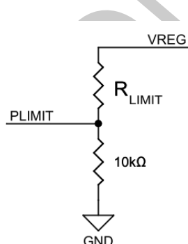
Figure 2. PLIMIT Pin Voltage Divider
