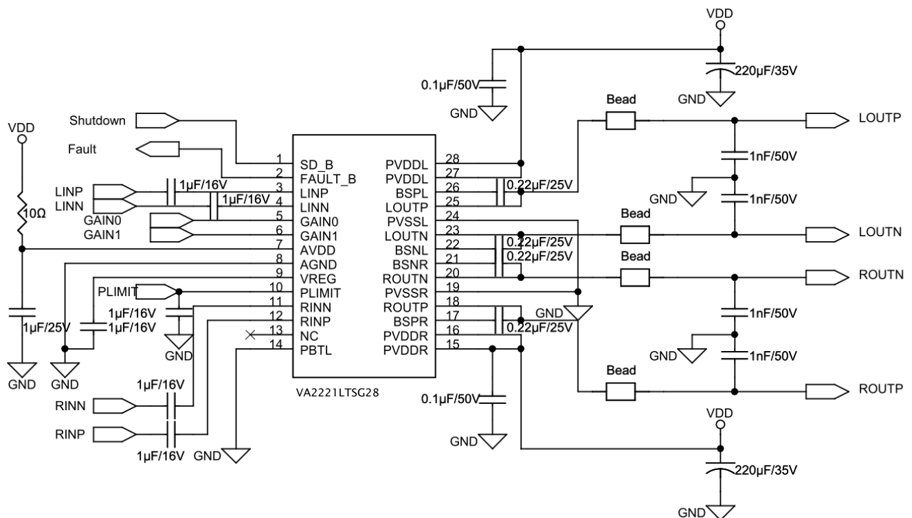
Figure 5. VA2221L Stereo Reference Application with Ferrite Bead
