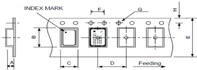
TAPE (CARRIER) DIMENSIONS
