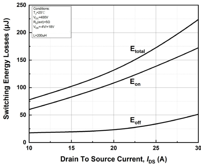
Figure 19. Clamped Inductive Switching Energy vs. Drain Current( V_{DS} = 400V )
