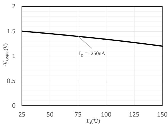
Fig 10 Gate Voltage vs. Junction Temperature
