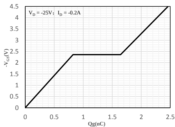
Fig 12 Gate-Charge Characteristics
