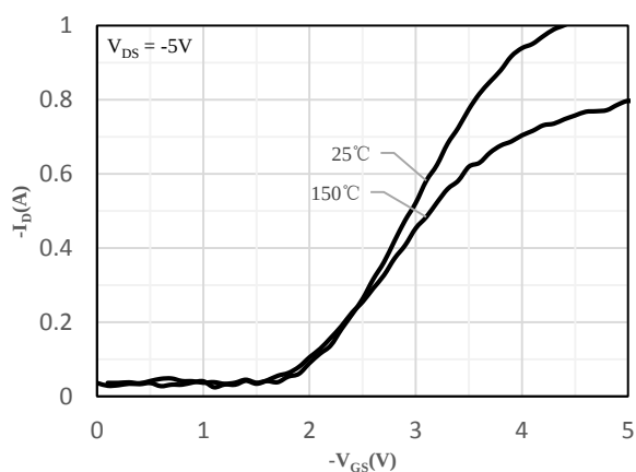
Fig 11 Transfer Characteristics
