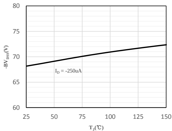
Fig 8 Drain-Source Voltage vs. Junction Temperature
