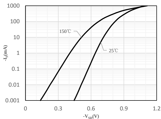
Fig 6 Body-Diode Characteristics
