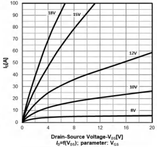
On-Region characteristics T_j=25\text{ }^\circ\text{C}
