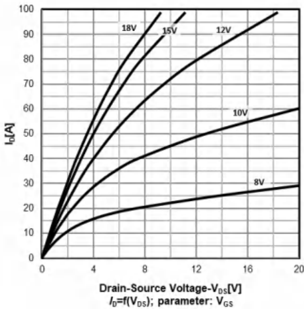
On-Region characteristics T_j=175\text{ }^\circ\text{C}
