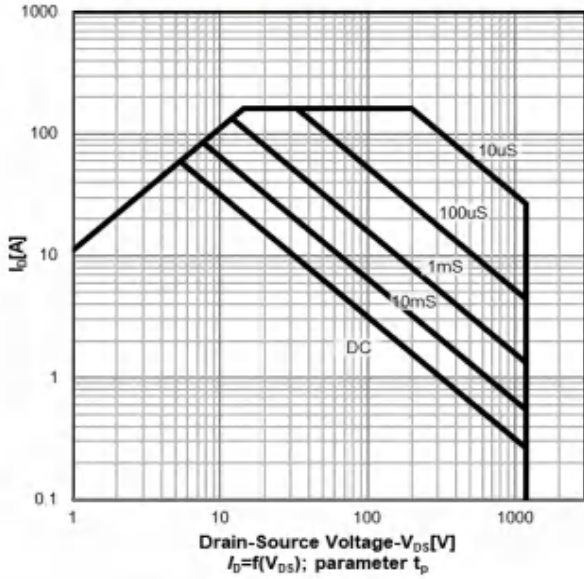
Safe operating area T_c=25\text{ }^\circ\text{C} TO-247
