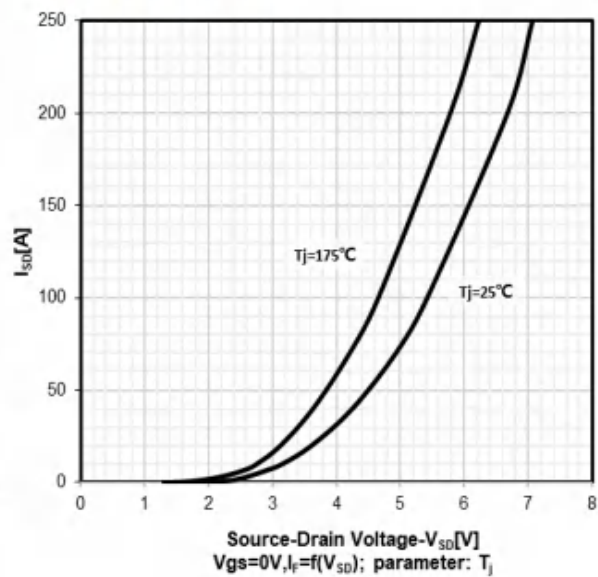
Diode forward voltage characteristics T j =25 °C/175 °C
