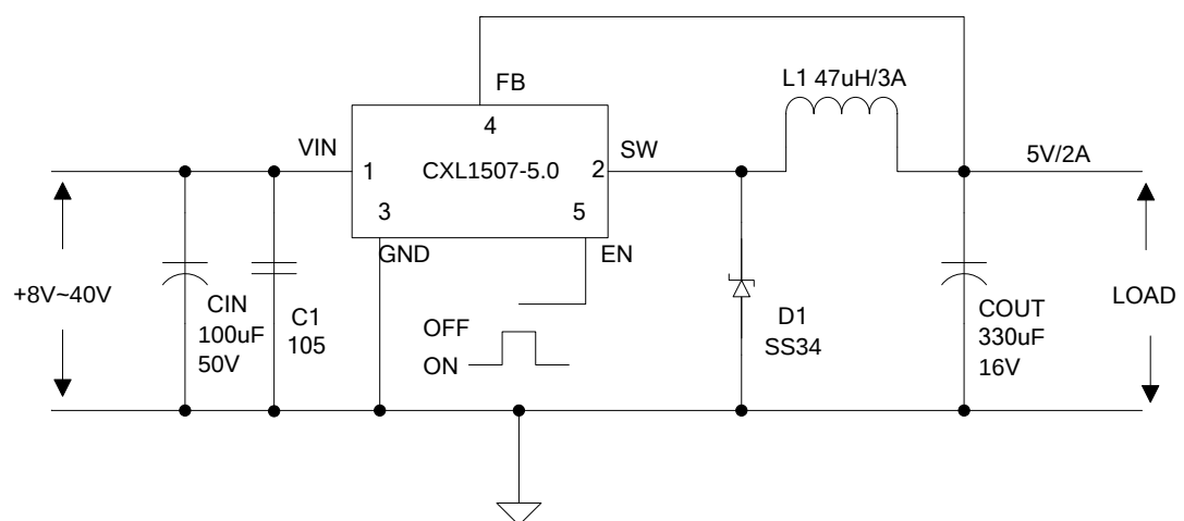
Figure4.CXL1507 Typcal Application Circuit(VIN=8V~40V.VOUT=5V/2A)
