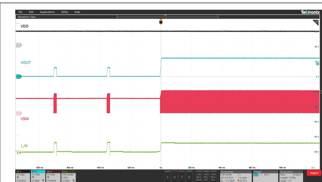
Figure 38. OCP Recovery at Heavy Load
