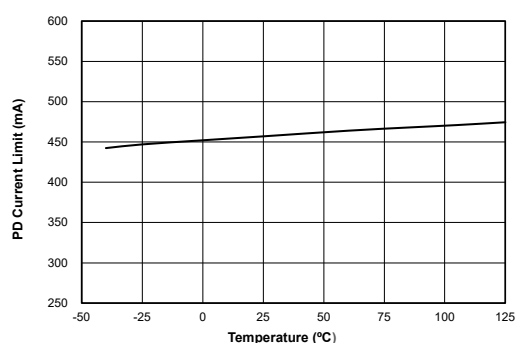
Figure 14. PD current Limit vs. Temperature
