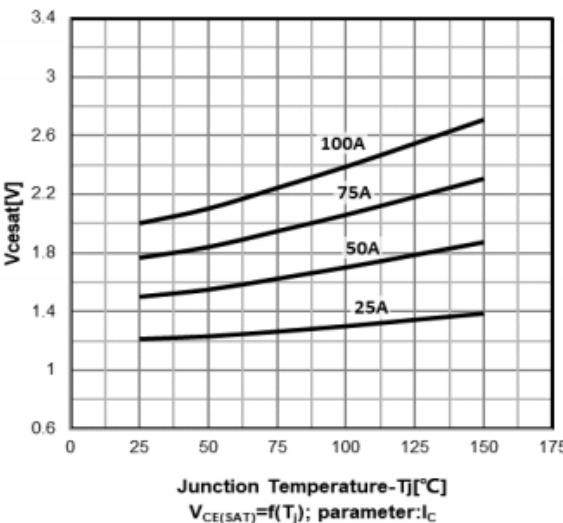
Typ. Collector-emitter saturation voltage as a function of junction temperature ( V_{GE} = 15\text{V} )
