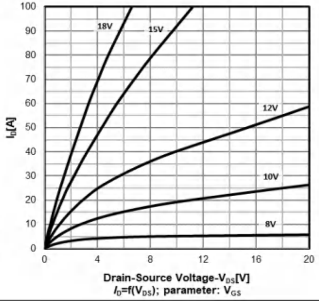
On-Region characteristics Tj=25 °C
