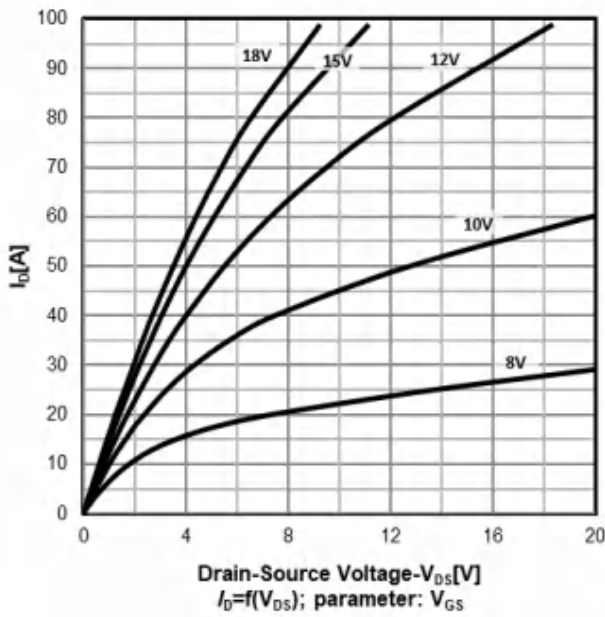
On-Region characteristics Tj=175 °C
