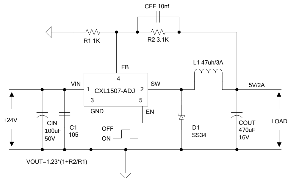
Figure8. CXL1507-ADJ System Parameters Test Ctrcuit
