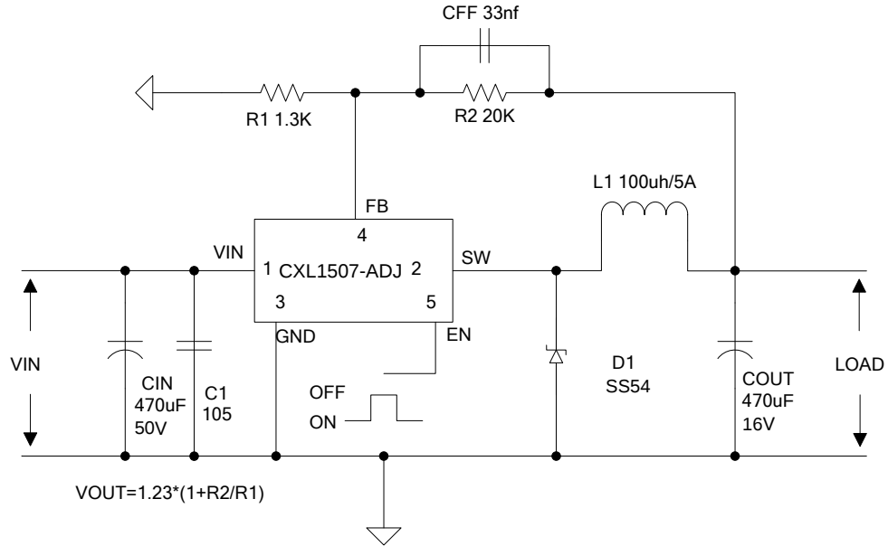
Figure9. CXL1507-ADJ High Power Applicationg Circuit( V_{IN}=24V . I_{OUT}=0.5A )
