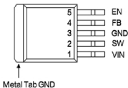
Figure 2 Pin Configuration of CXL1507(Top View)
