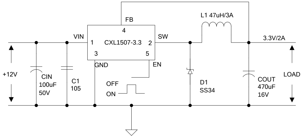
Figure5. CXL1507-3.3 System Parameters Test Ctrcuit
