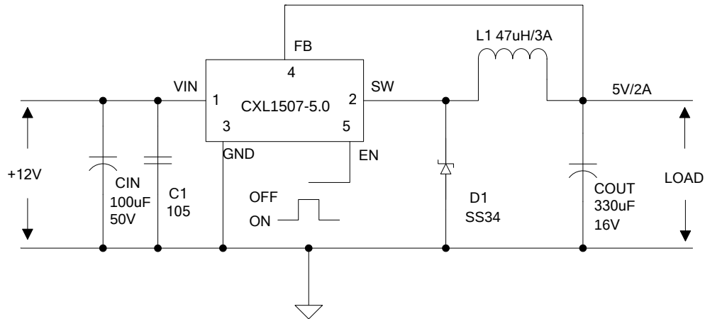
Figure6. CXL1507-5.0 System Parameters Test Ctrcuit
