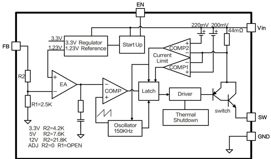
Figure 3 Function Block Diagram of CXL1507
