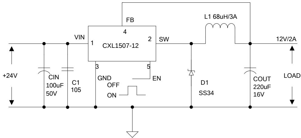
Figure7. CXL1507-12 System Parameters Test Ctrcuit
