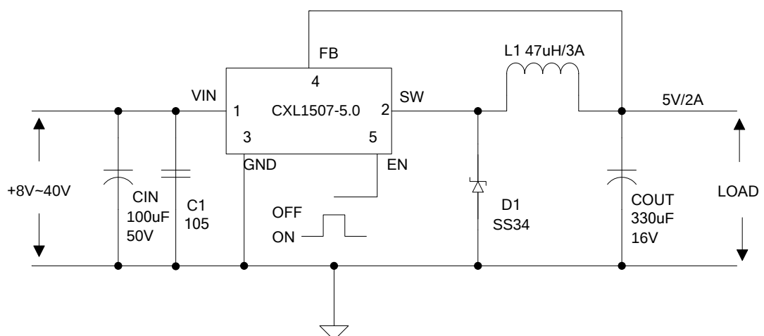
Figure4.CXL1507 Typical Application Circuit(VIN=8V~40V.VOUT=5V/2A)
