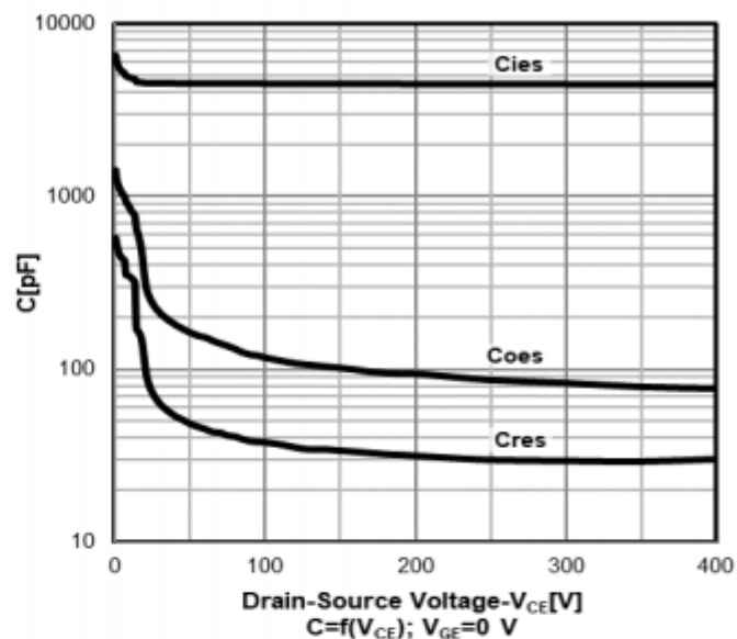
Capacitance characteristics
