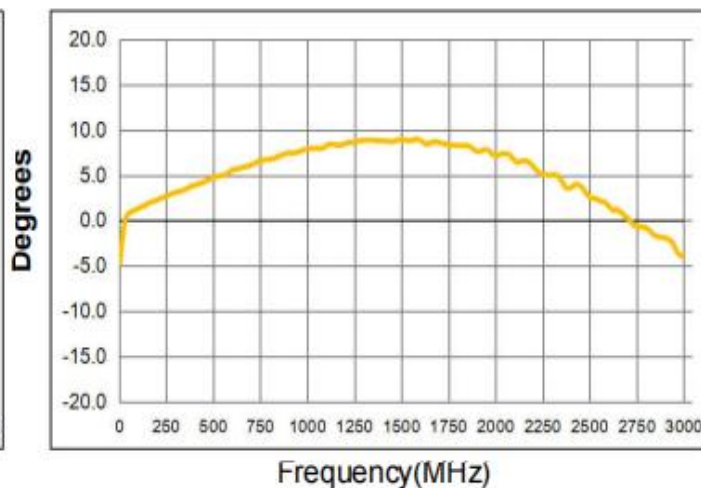
Phase Balance
