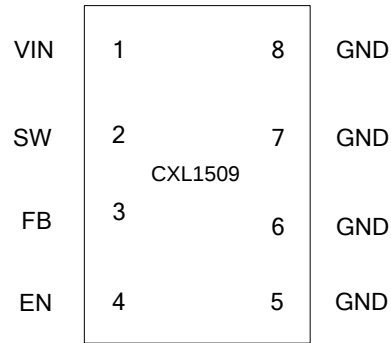
Figure 2 Pin Configuration of CXL1509 (Top View)
