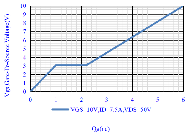
Fig.10-Gate Charge Waveform
