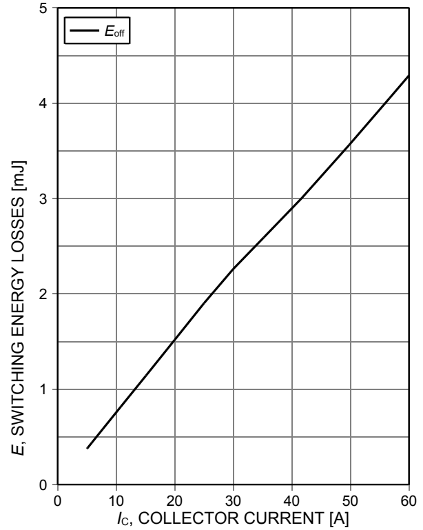
Figure 12. Typical switching energy losses as a function of collector current
