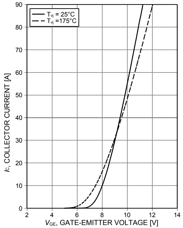
Figure 6. Typical transfer characteristic
