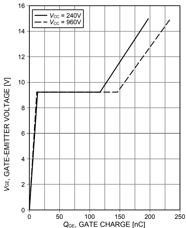
Figure 17. Typical gate charge
