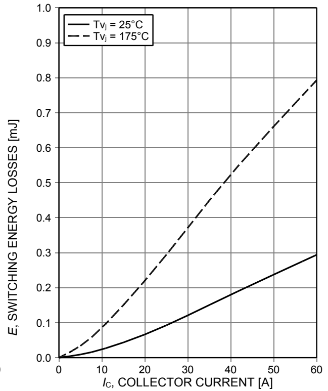
Figure 16. Typical turn off switching energy loss for soft switching
