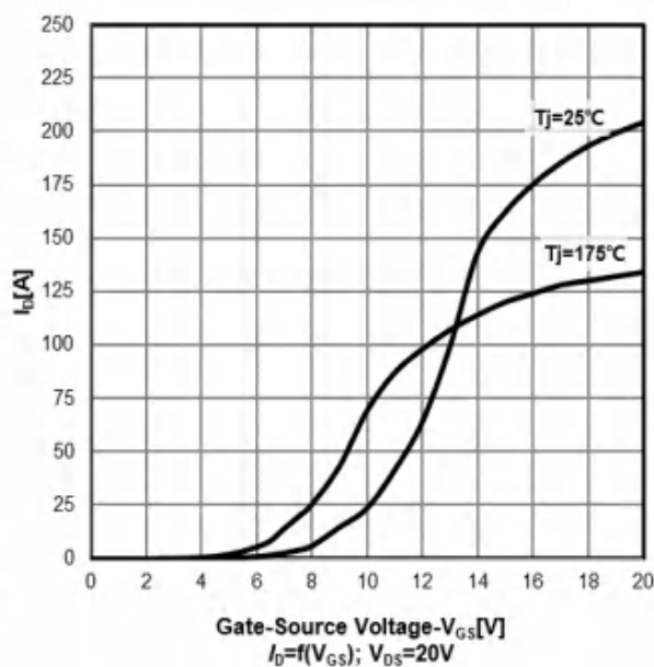
Transfer characteristics
