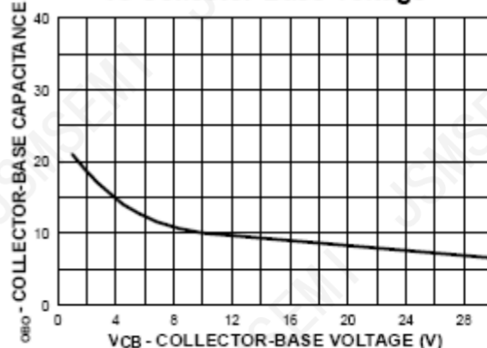
Collector-Base Capacitance vs Collector-Base Voltage
