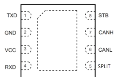
DFN-8 3*3
