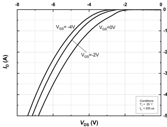
Figure 7. Body Diode Characteristics at T_j=25^{\circ}\text{C}
