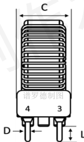
侧视图 side view
