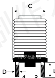
侧视图 side view
