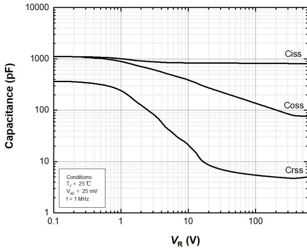
Figure 13. Capacitance vs. Drain-Source Voltage (0 – 600V)
