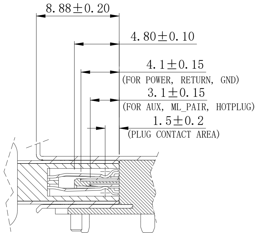
CONNECTOR MATING DIAGRAM
