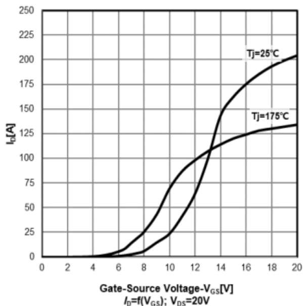
Transfer characteristics
