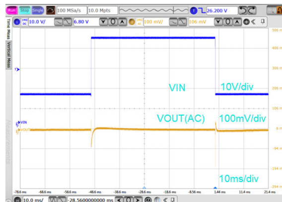
Figure 14. Line Transient
