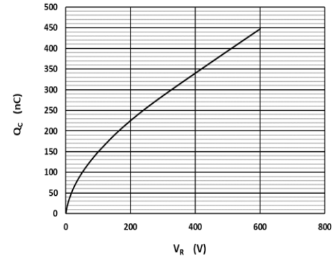
Fig 6: Reverse Charge vs. Reverse Voltage
