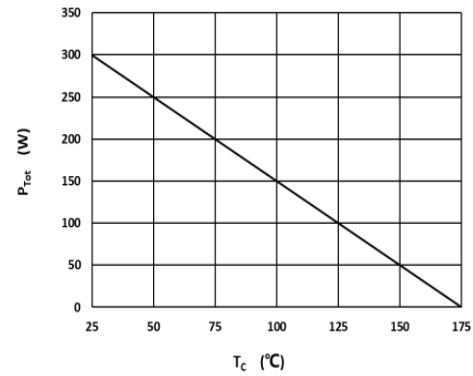
Fig 4: Power Derating
