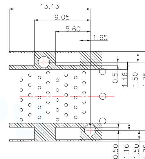
DETAIL-KEEPOUT ZONES
