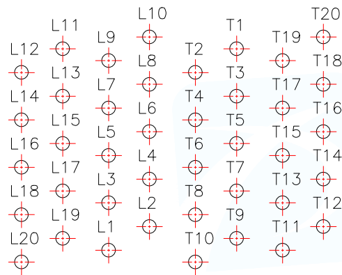
CIRCUT NUMBERING COMPONENT SDE OF BOARD
