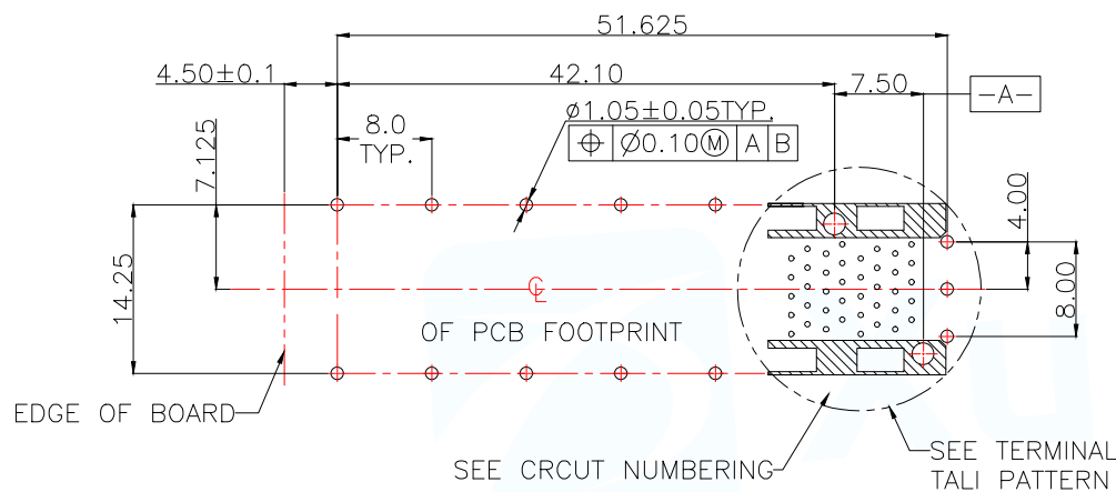
RECOMMENDED PCB LAYOUT – COMPONENT SIDE RECOMMENDED PCB THICKNESS:2.36MM(.093 INCH)
