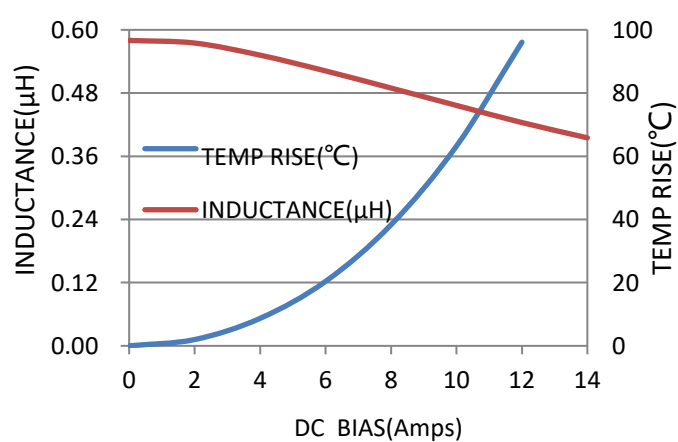
VCMA-0420-R56-M-1A
