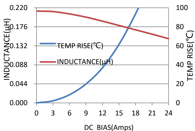
VCMA-0420-R22-M-1A
