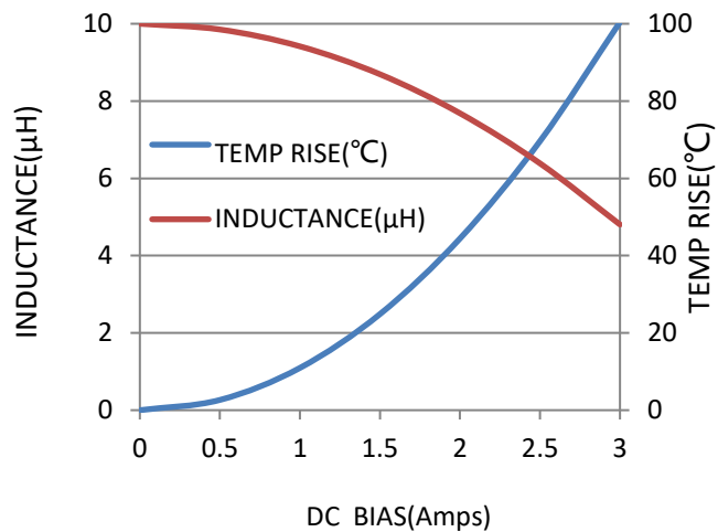
VCMA-0420-100-M-1A
