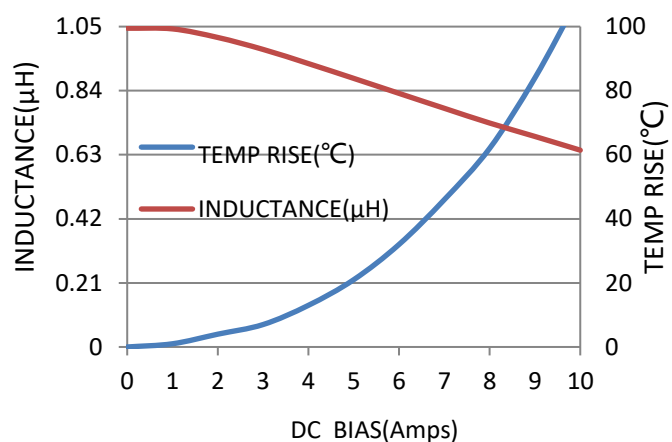
VCMA-0420-1R2-M-1A
