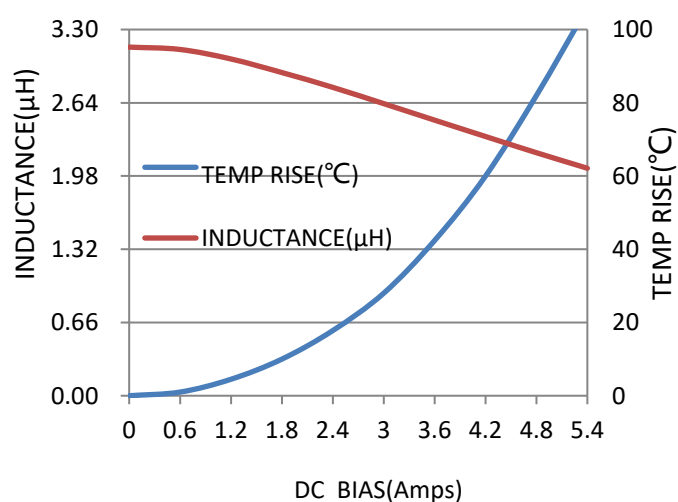
VCMA-0420-3R3-M-1A
