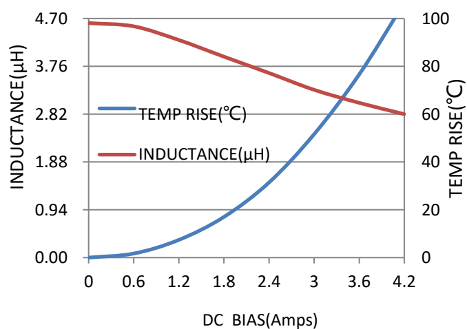
VCMA-0420-4R7-M-1A
