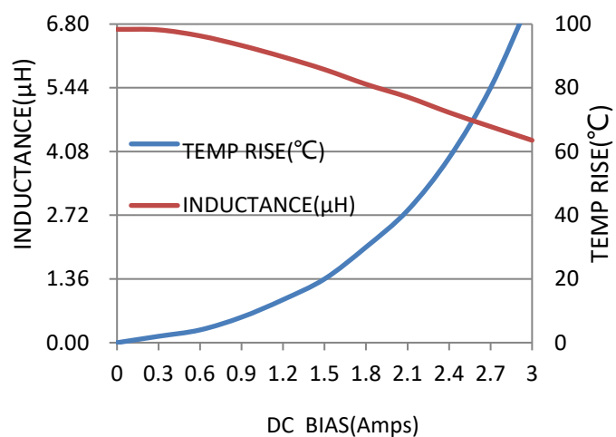
VCMA-0420-6R8-M-1A
