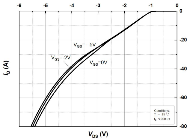
Figure 7. Body Diode Characteristics at T_J = 25^{\circ}C
