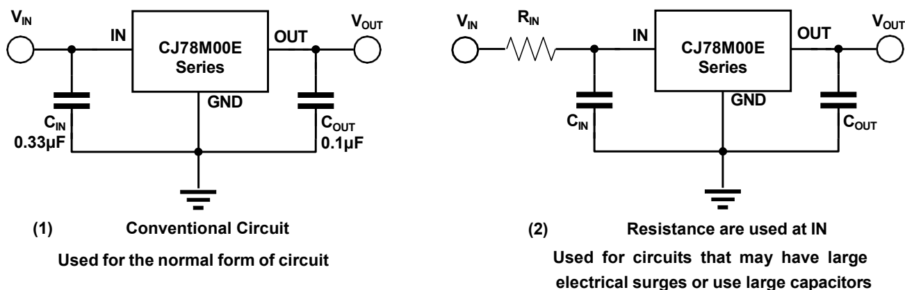
Figure 8-3. Fixed Output Regulator
