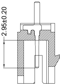
SECTION I-I
