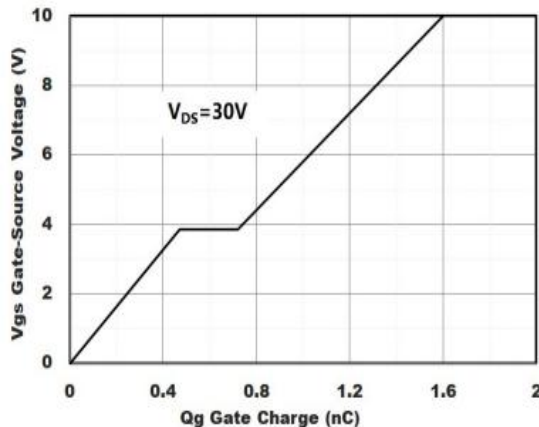
Figure 6: Gate-Charge Characteristics
